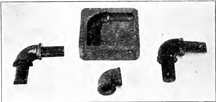
FIG. 575. CORE-BOX, PATTERN OF PIPE FITTING, ELBOW.
